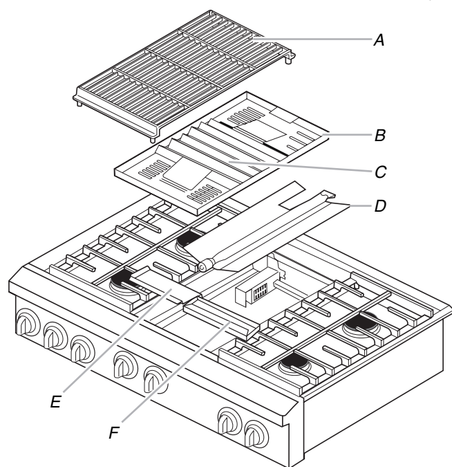
A. Grill grate B. Wave tray C. Wave plate
